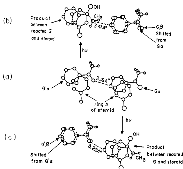
Figure 5. (a) Close-packed pair of G \alpha and G' \alpha molecules. Rings A of DCA related by c axis also shown. (b) Close-packed pair in which G' reacted. Its neighbor G \beta shifted along -c with respect to G \alpha to accommodate acceptable intermolecular distance of 3.4 Å. (c) Pair in which G reacted. Its neighbor G' \beta shifted along +c with respect to G' \alpha to accommodate acceptable intermolecular distance of 3.2 Å.
