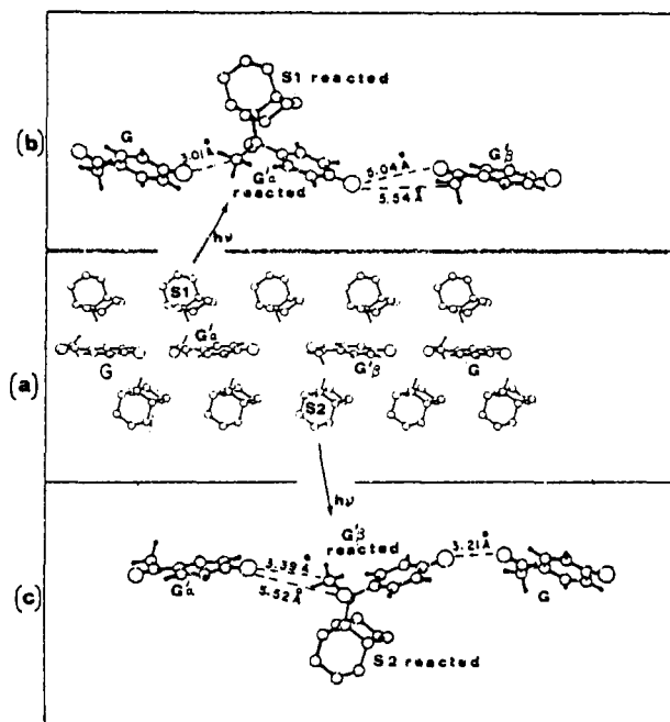
Figure 10. (a) Part of the chain of fluoracetophenone guest molecules sandwiched between rings A and B of the host DCA molecules in the unreacted crystal. The to-be-abstracted H5 atom attached to C5 of DCA is the only steroid H atom drawn. (b) Contacts between reacted G'α, bonded to steroid S1 and neighboring G and G'β molecules. (c) Contacts between reacted G'β, bonded to steroid S2 and neighboring G' and G molecules.
