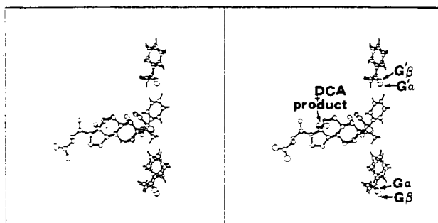
Figure 6. Stereoscopic view showing geometric relationship between overlapping unreacted DCA, photoproduct 1, and the position of the neighboring guest molecules. G \alpha and G' \alpha depict the positions of unreacted guest prior to reaction of a neighboring guest. G \beta and G' \beta are the corresponding positions after reaction of a neighboring guest.
