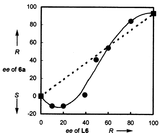
Figure 1. Enantioselectivity for the reaction of 4 with 5a catalyzed by the zinc complexes of partially resolved ( R )- L6 . The broken line indicates the expected values when the reactivity difference between Zn/( R )- L6 and Zn/( S )- L6 was not considered.
