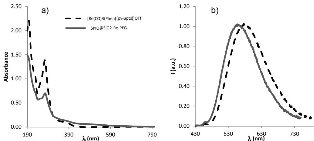
Fig. 2. a) UV-vis absorption and b) normalized photoluminescence spectra ( \lambda_{\text{ex}} = 375 nm) of [\text{Re}(\text{phen})(\text{CO})_3(\text{py-upts})]\text{OTf} (black dashed traces) and \text{SPIO@SiO}_2\text{-Re@PEG} (gray traces) in air equilibrated water solution at room temperature.
