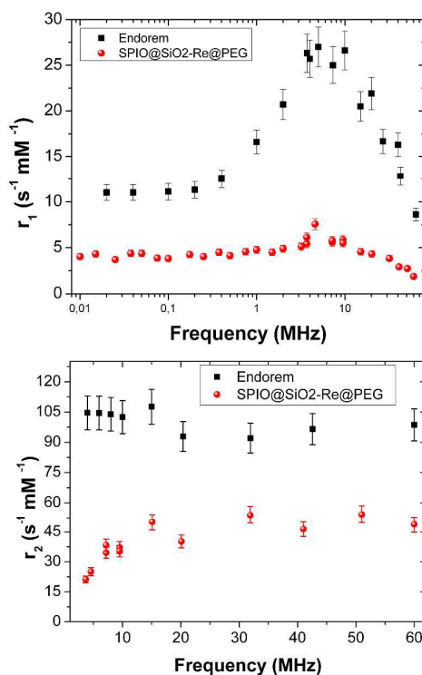
Fig. 3. Longitudinal (top) and transverse (bottom) relaxivities of SPIO@SiO 2 -Re@PEG nanoparticles (red circles) dispersed in water. Data are compared with the commercial compound Endorem® values (black squares).
