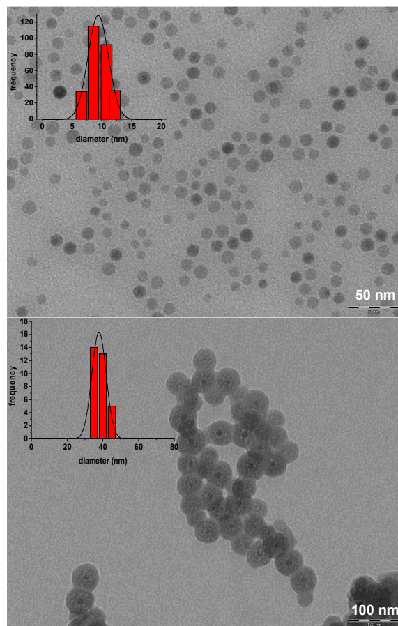
Fig. 1. TEM micrograph of the SPIO@OA nanoparticles (up) and of the core/shell SPIO@SiO 2 -Re@PEG nanoparticles (down), with the corresponding size distribution histograms.
