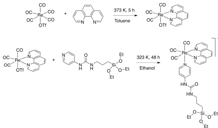
Scheme 2. Synthetic route to the complex [Re(phen)(CO) 3 (py-upts)]OTf.
