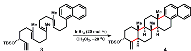
Scheme 2. In(III)-Catalyzed Enantioselective Cationic Polycyclization
