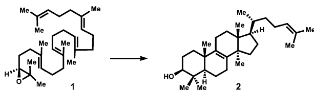
Scheme 1. Biosynthesis of Lanosterol
