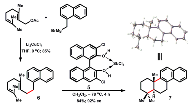
Scheme 3. Synthesis of Chiral Tetracycle
