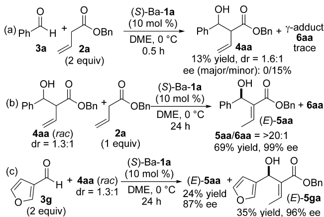
Scheme 2. Mechanistic Studies of Ba-Catalyzed DYKAT
