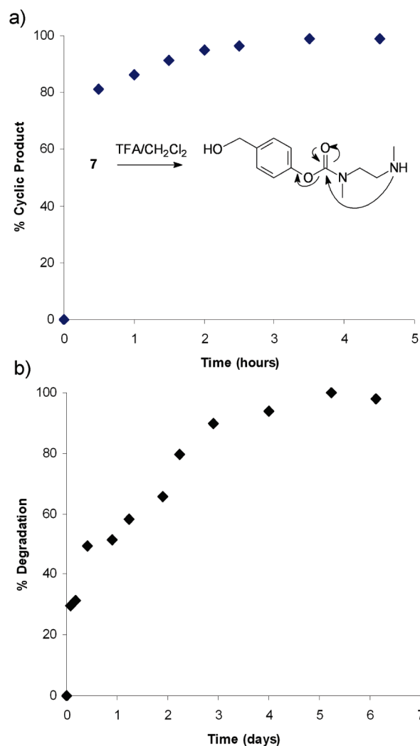
Figure 4. (a) Kinetics of cyclization of compound 7 , as measured by 1 H NMR spectroscopy in 0.1 M phosphate buffer (D 2 O):acetone- d 6 (3:2) at 37 °C, following removal of the Boc protecting group. (b) Kinetics of depolymerization of polymer 10 , as measured by 1 H NMR spectroscopy in 0.1 M phosphate buffer (D 2 O):acetone- d 6 (3:2), following removal of the Boc end-cap.
