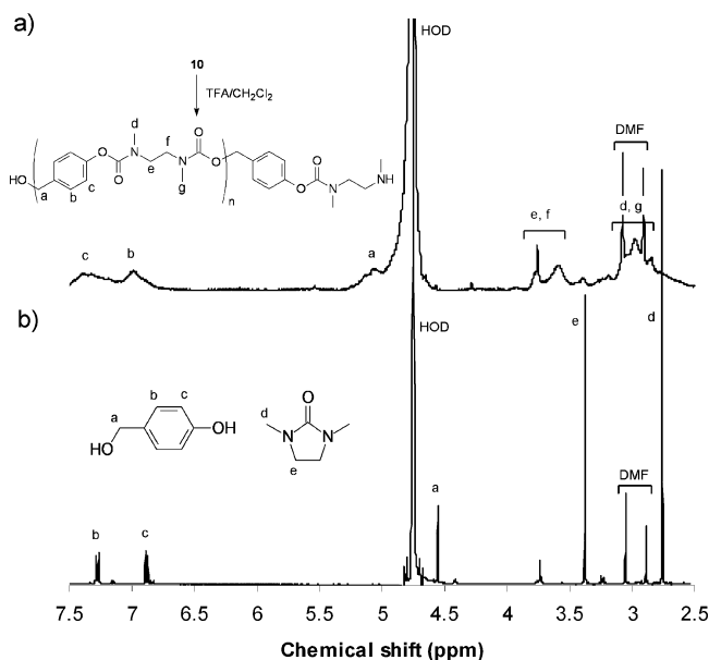
Figure 5. ^1\text{H} NMR spectra of (a) polymer 10 following end-cap removal in 0.1 M phosphate buffer ( \text{D}_2\text{O} ):acetone- d_6 (3:2) at t = 0 in the degradation process and (b) the same polymer solution after 5 days at 37^\circ\text{C} , showing complete depolymerization into small molecules.
