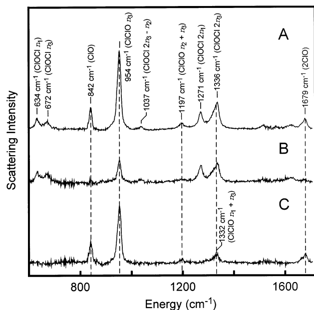
Figure 5. (A) Resonance Raman spectrum of ClOCl in CCl 4 obtained with 57 \mu J/pulse at 282.4 nm. Scattering due to ClOCl, ClCIO, and ClO is observed. (B) Resonance Raman spectrum of ClOCl in CCl 4 obtained with 6.7 \mu J/pulse at 282.4 nm. Scattering due to ClOCl is still present, but scattering due to ClCIO and ClO has diminished with the decrease in pulse energy. (C) Difference spectrum generated by subtracting (B) from (A) until the scattering due to ClOCl has vanished. This demonstrates that the only photoproducts of ClOCl are ClCIO and ClO.
