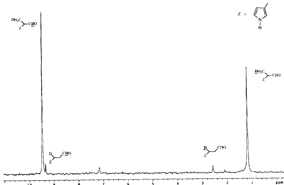
Fig. 3. ^2\text{H} NMR spectrum (46 MHz, 25°C, \text{C}_6\text{D}_6 as external standard) of the crude reaction mixture in benzene, obtained by deuterioformylation of the 3-vinylpyrrole ( 1c ) at 20°C.
