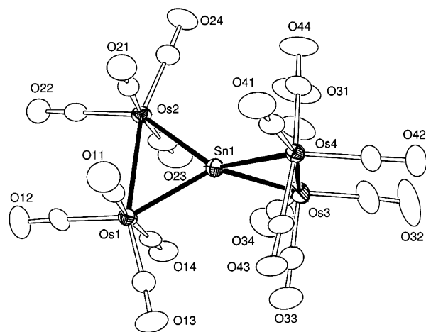
Figure 2. ORTEP diagram of \text{Os}_4(\text{CO})_{16}(\mu_4\text{-Sn}) , 9 , showing 30% probability thermal ellipsoids. Selected interatomic distances (Å) and angles (deg): Os(1)–Os(2) = 3.0081(5), Os(1)–Sn(1) = 2.6927(7), Os(2)–Sn(1) = 2.6883(7), Os(3)–Os(4) = 3.0038(5), Os(3)–Sn(1) = 2.6983(7), Os(4)–Sn(1) = 2.6797(7); Os(4)–Sn(1)–Os(2) = 136.86(3), Os(4)–Sn(1)–Os(1) = 135.85(2), Os(2)–Sn(1)–Os(1) = 67.975(17), Os(4)–Sn(1)–Os(3) = 67.907(18), Os(2)–Sn(1)–Os(3) = 130.34(3), Os(1)–Sn(1)–Os(3) = 130.32(2).
