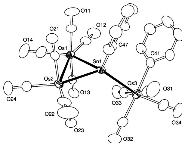
Figure 1. ORTEP diagram of \text{Os}_3(\text{CO})_{12}(\text{Ph})(\mu_3\text{-SnPh}) , 8 , showing 30% probability thermal ellipsoids. Selected interatomic distances (Å) and angles (deg): Os(1)–Os(2) = 3.0007(4), Os(1)–Sn(1) = 2.7240(6), Os(2)–Sn(1) = 2.7283(6), Os(3)–Sn(1) = 2.7532(6), Os(3)–C(41) = 2.172(9); Os(1)–Sn(1)–Os(3) = 126.597(19), Os(2)–Sn(1)–Os(3) = 128.81(2), C(41)–Os(3)–Sn(1) = 82.8(2).
