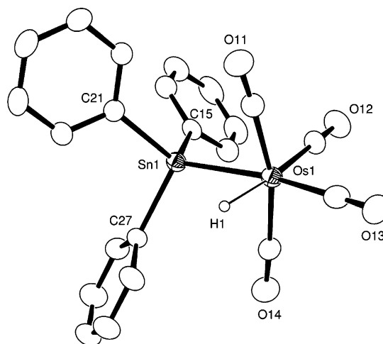
Figure 4. ORTEP diagram of \text{HOs}(\text{CO})_4(\text{SnPh}_3) , 11 , showing 30% probability thermal ellipsoids. Selected interatomic distances (Å) and angles (deg): \text{Os}(1)\text{--Sn}(1) = 2.7382(2) , \text{Os}(1)\text{--H}(1) = 1.67(4) , \text{Os}(1)\text{--C}(11) = 1.944(3) , \text{Os}(1)\text{--C}(12) = 1.967(3) , \text{Os}(1)\text{--C}(13) = 1.948(3) , \text{Os}(1)\text{--C}(14) = 1.942(3) ; \text{Sn}(1)\text{--Os}(1)\text{--H}(1) = 79.3(12) .
