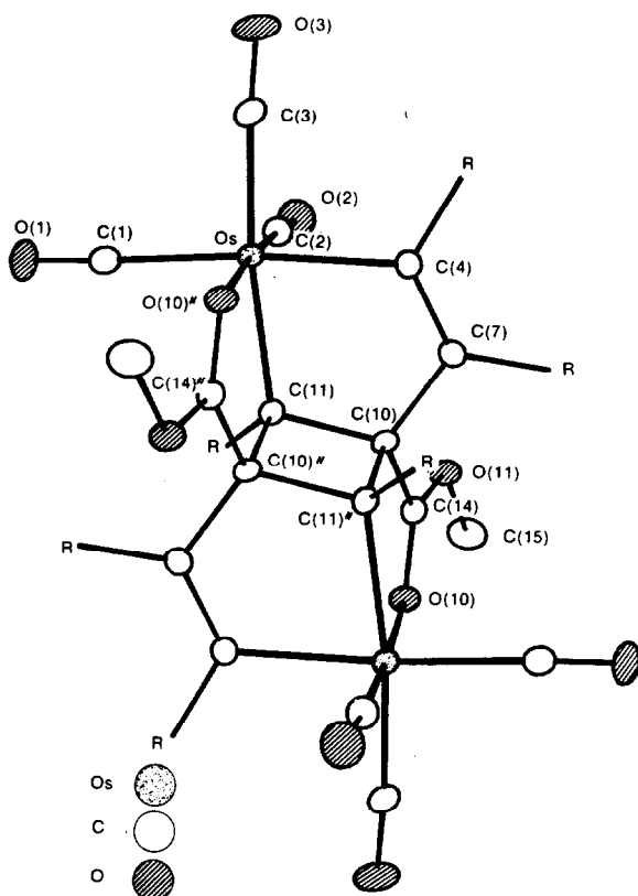
Fig. 2. Perspective view of \text{Os}_2(\text{CO})_6(\text{DMAD})_4 (5). Atoms are represented by thermal ellipsoids at the 20% probability level. For clarity some of the COOMe groups have been replaced by R. Selected average bond lengths (Å): Os—C(4) 2.101(5), Os—C(11) 2.156(5), Os—O(10) " 2.132(5), C(14)—O(10) 1.244(7), C—O (unbound) 1.189(7), C(4)—C(7) 1.350(8), C(7)—C(10) 1.490(7), C(10)—C(11) 1.578(7), C(10)—C(11) " 1.592(8). Selected average bond angles (deg): C(4)—Os—C(11) 79.8(2), C(11)—Os—O(10) " 80.0(2), Os " —O(10)—C(14) 116.8(4), C(10)—C(11)—C(10) " 90.7(4), C(11)—C(10)—C(11) " 89.3(4) (" indicates an atom centrosymmetrically related to the unprimed atom of the same name).
