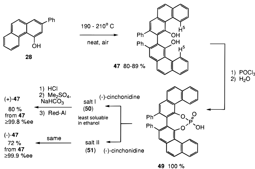
Scheme 10
