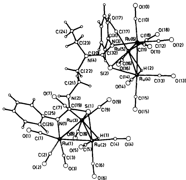
Fig. 1. View of the molecular structure of ((\mu\text{-H})\text{Ru}_3(\text{CO})_9)_2[\text{SC}(\text{NPh})\text{N}(\text{Et})(\text{CH}_2)_2\text{NH}(\text{PhN})\text{CS}] ( 4 ) together with the atomic numbering scheme.
