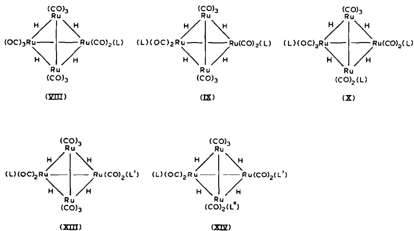
Fig. 1. Structures of complexes. Key to ligands used: (a) \text{PMe}_3 ; (b) \text{PMe}_2\text{Ph} ; (c) \text{PPh}_3 ; (d) \text{P}(\text{C}_6\text{H}_4\text{Me-}p)_3 ; (e) \text{P}(\text{C}_6\text{H}_4\text{Me-}o)_3 ; (f) \text{PCy}_3 ; (g) \text{P}(\text{CH}_2\text{CH}_2\text{CN})_3 ; (h) \text{P}(\text{OMe})_3 ; (i) \text{P}(\text{OMe})_2\text{Ph} ; (j) \text{P}(\text{OPh})_3 ; (k) \text{P}(\text{OC}_6\text{H}_4\text{Me-}p)_3 ; (l) \text{P}(\text{OCH}_2)_3\text{CEt} ; (m) \text{AsPh}_3 ; (n) \text{SbPh}_3 ; (o) \text{CNBu}' ; (p) \text{CNCy} ; (q) (+)-( R )- \text{CNCHMePh} ; (r) \text{CNCH}_2\text{SO}_2\text{C}_6\text{H}_4\text{Me-}p (tosmic); (s) \text{CH}_2(\text{PPh}_2)_2 (dppm); (t) \text{Ph}_2\text{PCH}_2\text{CH}_2\text{PPh}_2 (dppe); (u) \text{CH}_2(\text{AsPh}_2)_2 (dpam); (v) \text{Ph}_2\text{AsCH}_2\text{CH}_2\text{AsPh}_2 (dpae)
