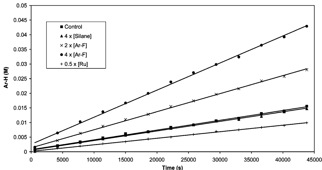
Figure 5. Time course plot of the catalytic HDF of \text{C}_6\text{F}_5\text{H} by \text{Ru}(\text{IPr})(\text{PPh}_3)_2(\text{CO})\text{H}_2 15 (THF, 339 K) showing changes in the initial rates upon varying the concentrations of \text{C}_6\text{F}_5\text{H} , \text{Et}_3\text{SiH} and 15 versus a standard experiment ( [\text{Et}_3\text{SiH}] = [\text{C}_6\text{F}_5\text{H}] = 0.1 \text{ M} , [\text{15}] = 0.01 \text{ M} ).
