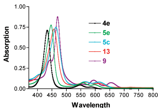
Figure 2. UV–vis absorption spectra of 4e , 5e , 5c , 9 , and 13 in \text{CH}_2\text{Cl}_2 .
