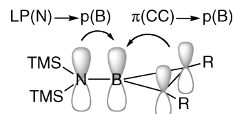
Figure 5. Schematic representation of the two-electron stabilizing donation to the p_z -atomic orbital at boron atom in borirenes 3–10 .
