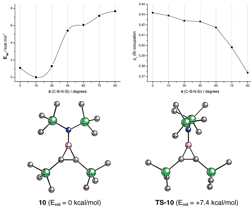
Figure 2. (Top) Relative energy of [(\mu\text{-BN}(\text{SiMe}_3)_2(\text{Me}_3\text{SiC}=\text{CSiMe}_3)] (left) and boron p_z orbital occupation (right) as a function of the dihedral angle between the \text{BNSi}_2 and \text{BC}_2 planes. (Bottom) Ball and stick representations of the calculated structures at the energy minimum (left) and transition state for B–N bond rotation (right). Hydrogen atoms were omitted for clarity.
