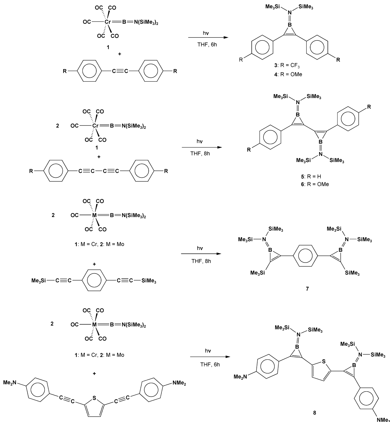
Scheme 2. Synthesis of Mono- and Bis-bis-(trimethylsilyl)aminoborirenes, from Borylene Complexes, [(\text{CO})_5\text{M}=\text{B}=\text{N}(\text{SiMe}_3)_2] ( \text{M} = \text{Cr} and \text{Mo} )
