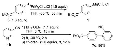
Scheme 3. Selective Addition of a Functionalized Grignard Reagent to Nicotinonitrile
