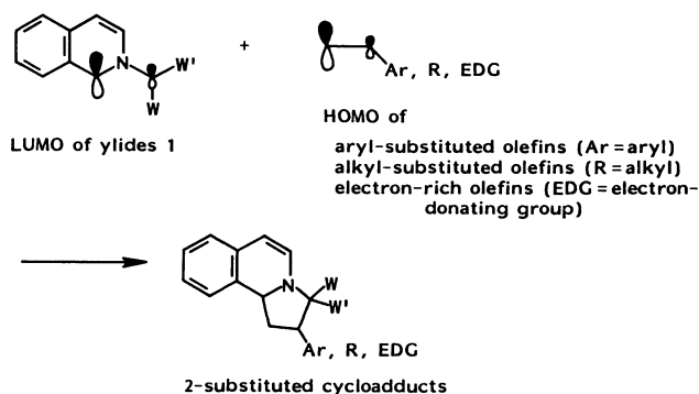
Fig. 4. LUMO ylide -HOMO dipolarophile interaction leading to regioselective cycloadducts.
