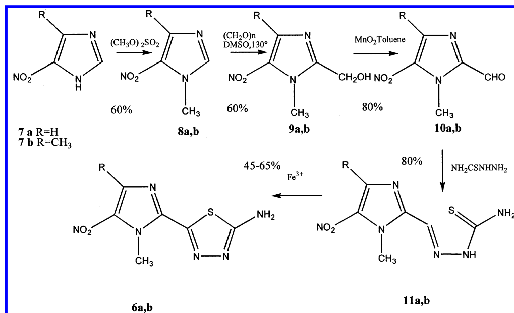
Figure 2. Synthesis of 4-methyl-megazol by the cyanamid procedure.
