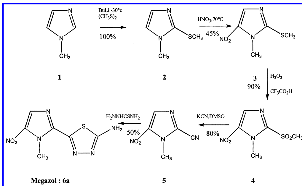
Figure 1. New procedure for megazol synthesis.
