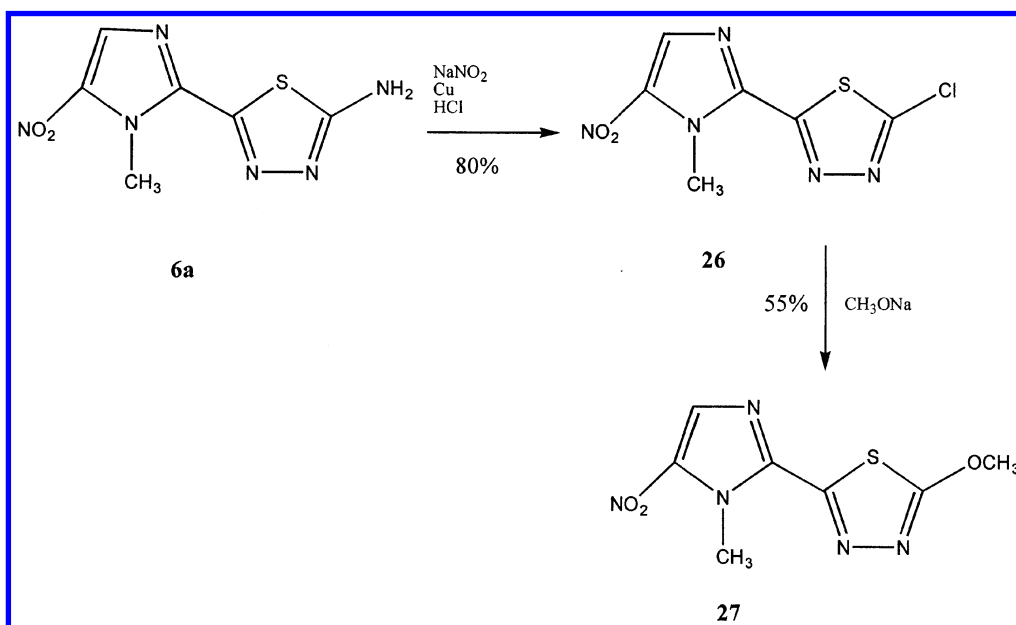
Figure 7. Substitutions of the amino group in the thiadiazole ring of megazol.
