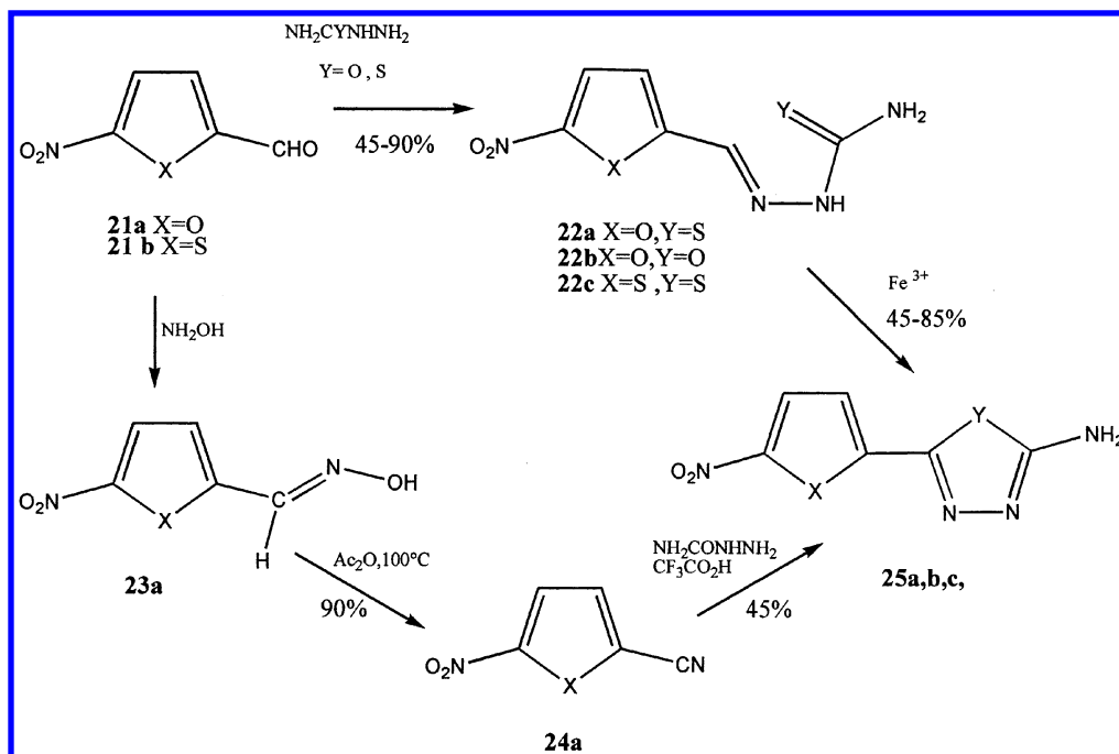
Figure 6. Route to analogues of megazol with nitrofurane and nitrothiophene in place of nitroimidazole.
