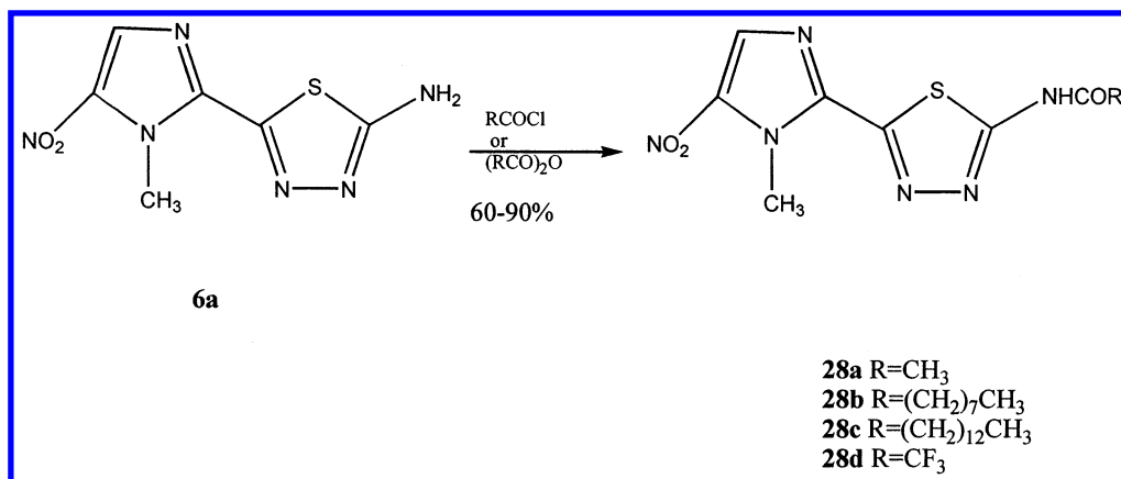
Figure 8. Synthesis of the alkylamides of megalol.
