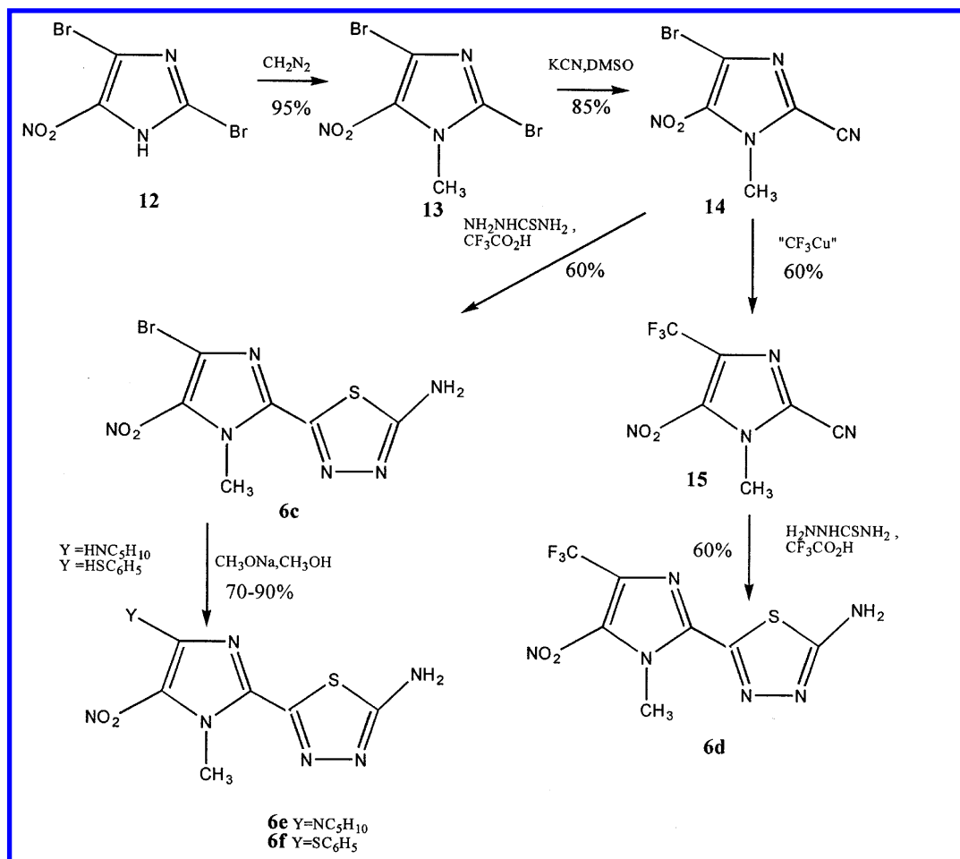
Figure 3. Synthesis of 4-substituted analogues of megazol.
