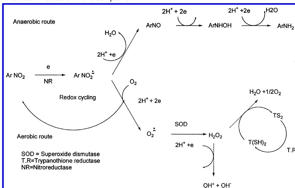
Scheme 1. Bioreduction Routes for Nitro Compounds
