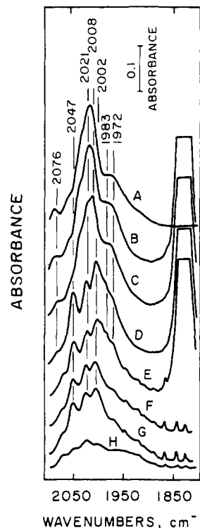
Figure 7. Infrared spectra showing the effect of but-1-ene on a sample prepared by adsorption of [\text{H}_2\text{RuOs}_3(\text{CO})_{13}] on \gamma\text{-Al}_2\text{O}_3 : (A) fresh sample at 25 °C under vacuum, (B) sample at 25 °C under but-1-ene + He, (C) after heating to 90 °C under but-1-ene + He, (D) after 1 h, (E) after 16 h under but-1-ene + He, (F) after evacuation at 90 °C, (G) at 25 °C under vacuum after cooling in CO, (H) sample at 25 °C under vacuum after extraction with \text{Et}_4\text{NBr} in \text{CH}_2\text{Cl}_2 .
