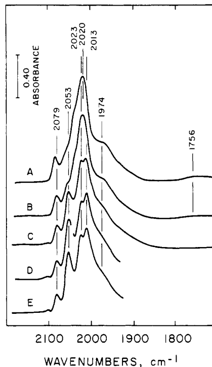
Figure 4. Infrared evidence of the conversion of [\text{HRuOs}_3(\text{CO})_{13}]\text{-[Al]} into [\text{H}_3\text{RuOs}_3(\text{CO})_{12}]\text{-[Al]} . The sample was prepared from [\text{H}_2\text{RuOs}_3(\text{CO})_{13}] and \gamma\text{-Al}_2\text{O}_3 pretreated at 110 °C: (A) fresh sample at 25 °C under vacuum, indicative of [\text{HRuOs}_3(\text{CO})_{13}]\text{-[Al]} , (B) after heating to 50 °C in He, (C) after 3 h at 50 °C in He, (D) after temperature had been raised to 70 °C with sample in He, and (E) sample under vacuum at 25 °C after 1 h at 70 °C in He. The final spectrum is that of [\text{H}_3\text{RuOs}_3(\text{CO})_{12}]\text{-[Al]} .
