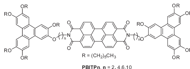
Figure 1. Target triphenylene–perylene–triphenylene triads PBITP n .
