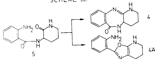
SCHEME III.
