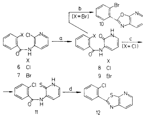
SCHEME IV.
