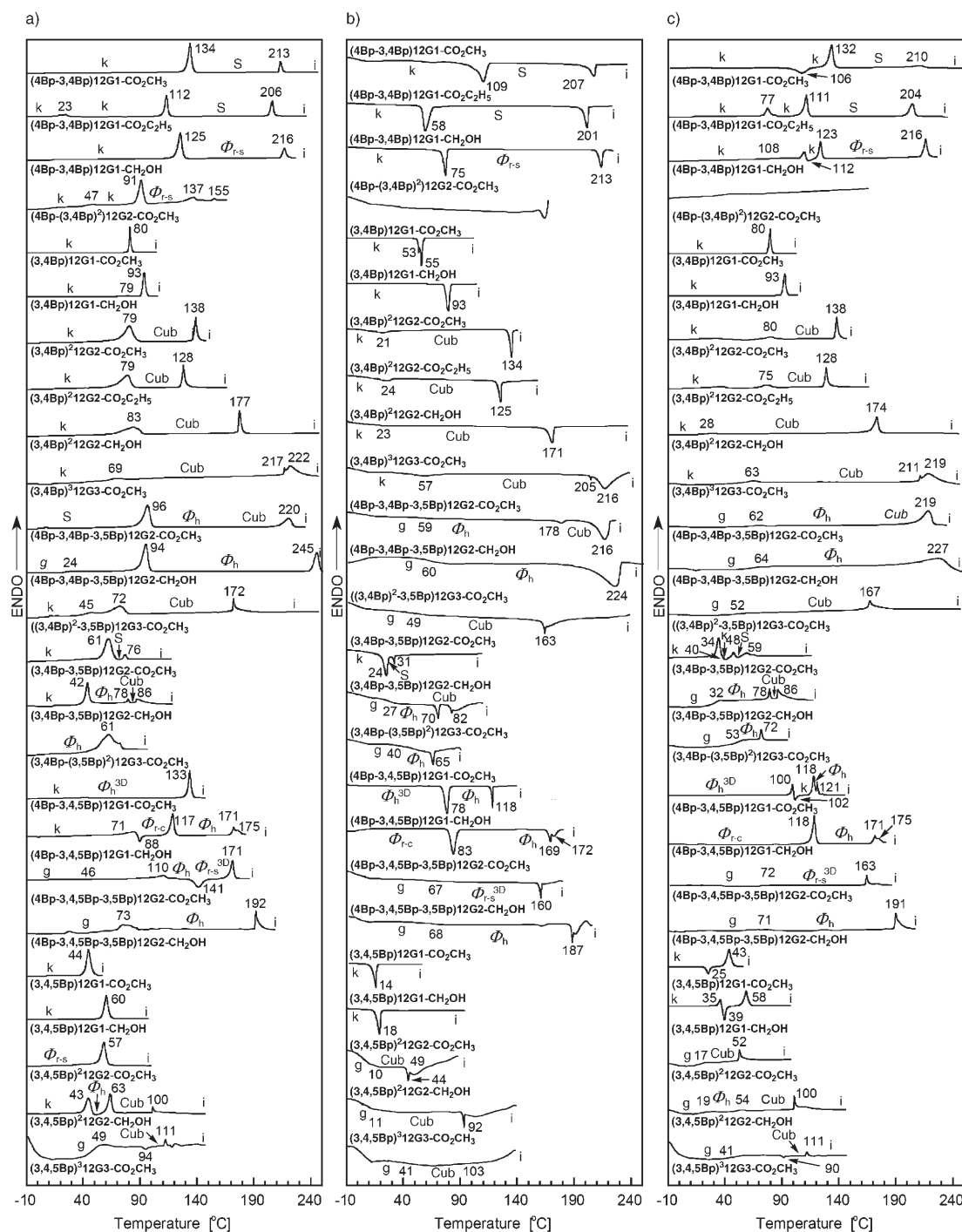
Figure 1. DSC traces [ 10^{\circ}\text{C}\cdot\text{min}^{-1} ] of biphenyl-based dendrons. Transition temperatures [ ^{\circ}\text{C} ] are marked on each trace: (a) first heating scan; (b) first cooling scan; (c) second heating scan. Peak intensities are not scaled.
