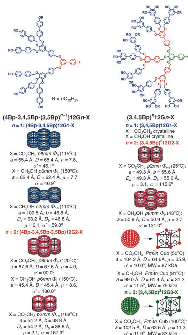
Scheme 8. Retrostructural analysis of supramolecular dendrimers self-assembled from 3,5-disubstituted AB 2 and 3,4,5-trisubstituted AB 3 biphenyl based dendrons.
