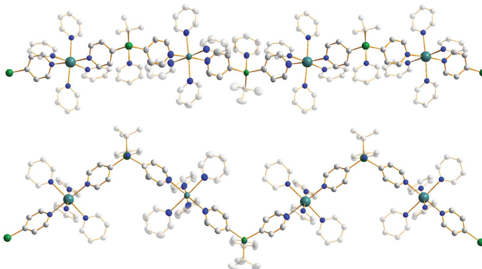
Fig. 7 Propagation of \{[Na \cdot 4py][Zn(py^*)_2(tBu) \cdot pyl]_\infty ( 3 ) into a polymer shown from the side and above. Ellipsoids are shown at 50% probability, all hydrogen atoms have been removed and all tBu carbon atoms and neutral donor pyridine ligands are highly transparent for clarity.
