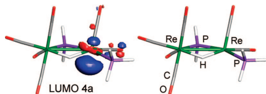
Figure 6. Contour diagram of the lowest unoccupied orbital LUMO 4a ( -2.95 eV) in 4 is shown on the left. A line structure showing the orientation of the molecule and the locations of the atoms in the MO diagram is shown on the right.
