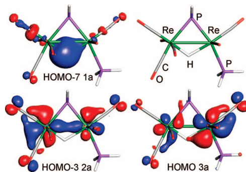
Figure 5. Contour diagrams for some selected Fenske-Hall molecular orbitals for 4 . HOMO-7 1a ( -12.25 eV), HOMO-3 2a ( -9.05 eV), HOMO 3a ( -7.42 eV). A line structure showing the locations of the atoms in the diagrams is shown at the top right.
