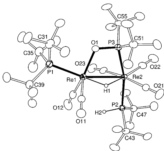
Figure 8. ORTEP showing the molecular structure of 5 at 30% thermal ellipsoid probability. Selected interatomic bond distances (Å) and angles (deg) are as follows: \text{Re}_1\text{--Re}_2 = 3.2048(4) , \text{Re}_1\text{--O}_1 = 2.067(5) , \text{Re}_1\text{--P}_1 = 2.457(2) , \text{Re}_1\text{--H}_1 = 1.67(8) , \text{Re}_2\text{--P}_3 = 2.4329(18) , \text{Re}_2\text{--P}_2 = 2.4688(18) , \text{Re}_2\text{--H}_1 = 1.93(7) , \text{P}_2\text{--H}_2 = 1.39(6) , \text{Re}_1 \cdots \text{C}_23 = 3.198 , \text{Re}_1 \cdots \text{O}_23 = 3.745(1) ; \text{P}_3\text{--Re}_2\text{--P}_2 = 165.56(6) , \text{O}_1\text{--P}_3\text{--Re}_2 = 105.19(19) , \text{P}_3\text{--O}_1\text{--Re}_1 = 115.4(3) .
