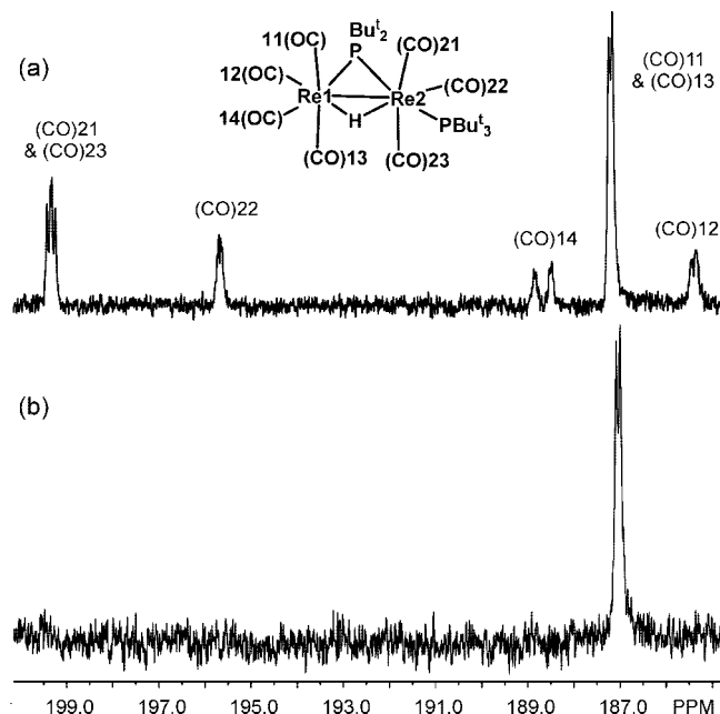
Figure 11. (a) ^{13}\text{C}\{^1\text{H}\} NMR spectrum of 6 having all CO sites enriched to \sim 30\% with ^{13}\text{CO} . (b) ^{13}\text{C}\{^1\text{H}\} NMR spectrum of 6 formed by the addition of ^{13}\text{CO} to a sample of 4 containing CO at the natural abundance level.
