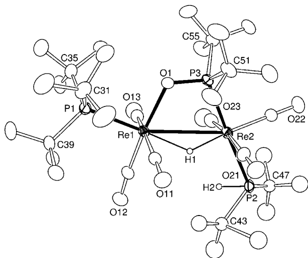
Figure 14. ORTEP showing the molecular structure of 9 at 30% thermal ellipsoid probability. Selected interatomic bond distances (Å) and angles (deg) are as follows: Re1–Re2 = 3.3711(5), Re1–O1 = 2.185(6), Re1–P1 = 2.539(2), Re2–P3 = 2.465(2), Re2–P2 = 2.522(6), P3–O1 = 1.565(6), Re1–H1 = 2.10(9), Re2–H1 = 1.66(9); P3–Re2–P2 = 172.42(15), P2–Re2–Re1 = 103.92(15), O1–P3–Re2 = 108.7(2), P3–O1–Re1 = 117.1(3).
