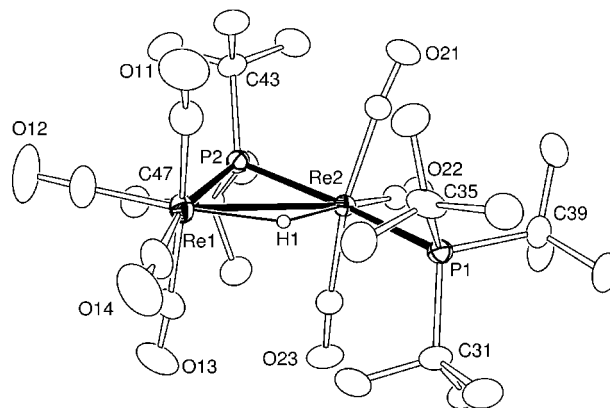
Figure 10. ORTEP of the molecular structure of 6 showing 30% thermal ellipsoid probability. Selected interatomic bond distances ( \text{\AA} ) and angles ( ^\circ ) are as follows: Re1–Re2 = 3.17813(18), Re1–P2 = 2.4871(9), Re2–P2 = 2.4461(8), Re2–P1 = 2.5931(8), Re1–H1 = 1.93(4), Re2–H1 = 1.87(4); C31–P1–Re2 = 113.76(12), C39–P1–Re2 = 111.62(12), C35–P1–Re2 = 110.16(14).
