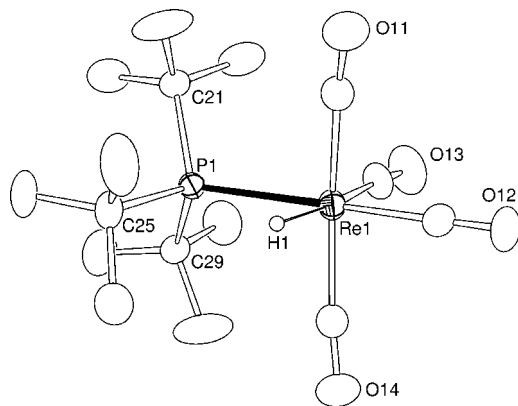
Figure 3. ORTEP showing the molecular structure of 3 at 30% thermal ellipsoid probability. Selected interatomic bond distances (Å) and angles (deg) are as follows: \text{Re1-H1} = 1.62(4) , \text{Re1-P1} = 2.5795(12) , \text{P1-Re1-H1} = 77.4(16) , \text{C12-Re1-P1} = 173.82(18) .
