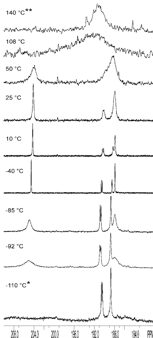
Figure 7. Variable-temperature ^{13}\text{C}\{^1\text{H}\} NMR spectra for compound 4 in d_8 -toluene solvent. *The spectrum at -110^\circ\text{C} was recorded in diethyl ether solvent with a drop of \text{CD}_2\text{Cl}_2 . **The spectrum at 140^\circ\text{C} was recorded in xylene solvent with a drop of d_8 -toluene.
