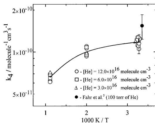
Figure 3. C 2 H 3 + CH 3 overall rate constants vs 1000 K/T. Current study: open circles, [He] = 12.0 × 10 16 molecules cm -3 ; squares, [He] = 6.0 × 10 16 molecules cm -3 ; triangles, [He] = 3.0 × 10 16 molecules cm -3 . Uncertainties (see Table 1) are not shown on the plot (except for one point) to avoid congestion. Solid line represents fitting of the experimental results with formula IV (no pressure dependence is assumed). Filled circle, result of Fahr et al. 5 (obtained at room temperature and 13.3 kPa (100 Torr) of He).
