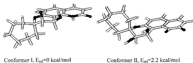
Fig. 2. Representation of the Low Energy Conformations for Derivative 21c Derived from Molecular Mechanics Calculations
