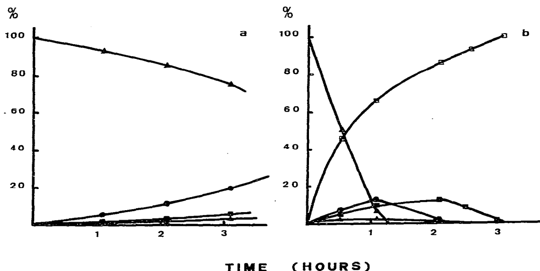
Fig. 3. Hydrogenation of 2-pentyne catalysed by \text{Rh}_2(\text{CO})_4\text{Cl}_2 (a) and \text{Rh}_2(\text{CO})_4\text{Cl}_2/\text{Al}_2\text{O}_3 (b) at 80^\circ\text{C} . \blacktriangle 2-pentyne; \bullet 2-cis-pentene; \blacksquare 2-trans-pentene; \triangle 1-pentyne; \square pentane.
