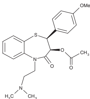
Figure 1. Diltiazem.
