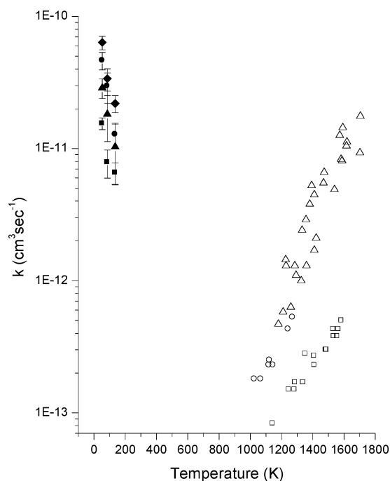
Figure 8. Temperature dependence of \text{NH} + \text{unsaturated hydrocarbons} . Filled symbols from this work: ◆ – diacetylene, ● – propene, ▲ – acetylene, ■ – ethylene. Open symbols from Rohrig et al. 11,12 using a shock tube apparatus. ○ – propene, △ – acetylene, □ – ethylene.
