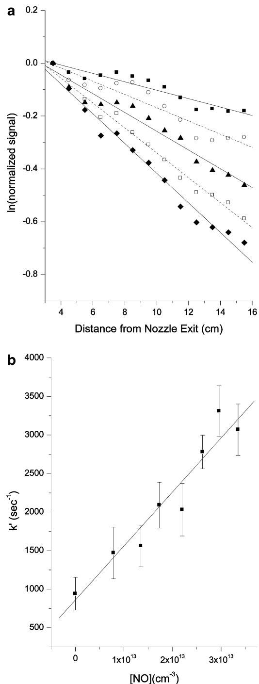
Figure 5. (a) Pseudo 1 st order decays for NH + NO in the N2M32e16 nozzle. Percent NO in flow: ■ – 0.00, ○ – 0.05, ▲ – 0.10, □ – 0.15, ◆ – 0.17. (b) Plot of k' vs [NO] used to extract the bimolecular rate coefficient.
