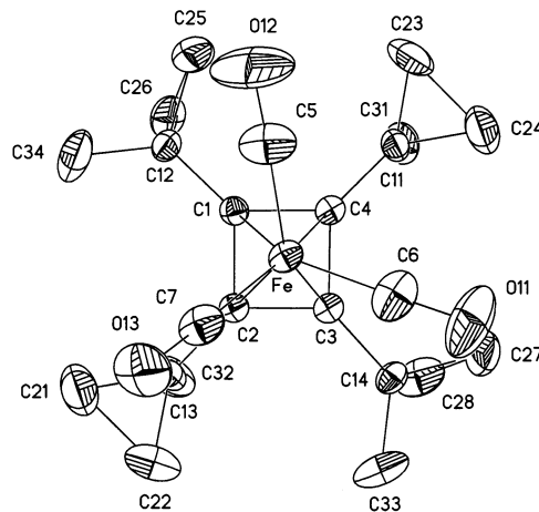
Fig. 1. Structure of tricarbonyl[tetrakis(1'-methylcyclopropyl)cyclobutadiene]iron ( 7 ) in the crystal.
