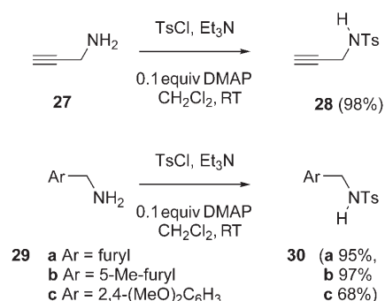
Scheme 6. Crystalline intermediates of the syntheses of substrates 1 .
