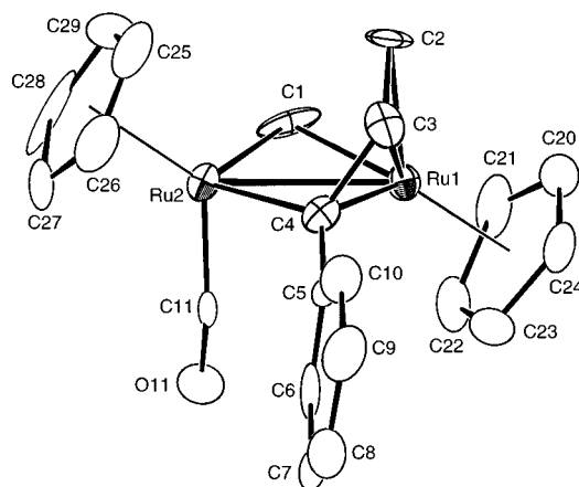
Figure 5. Molecular structure of 12a (molecule 1) drawn at the 30% probability level.
