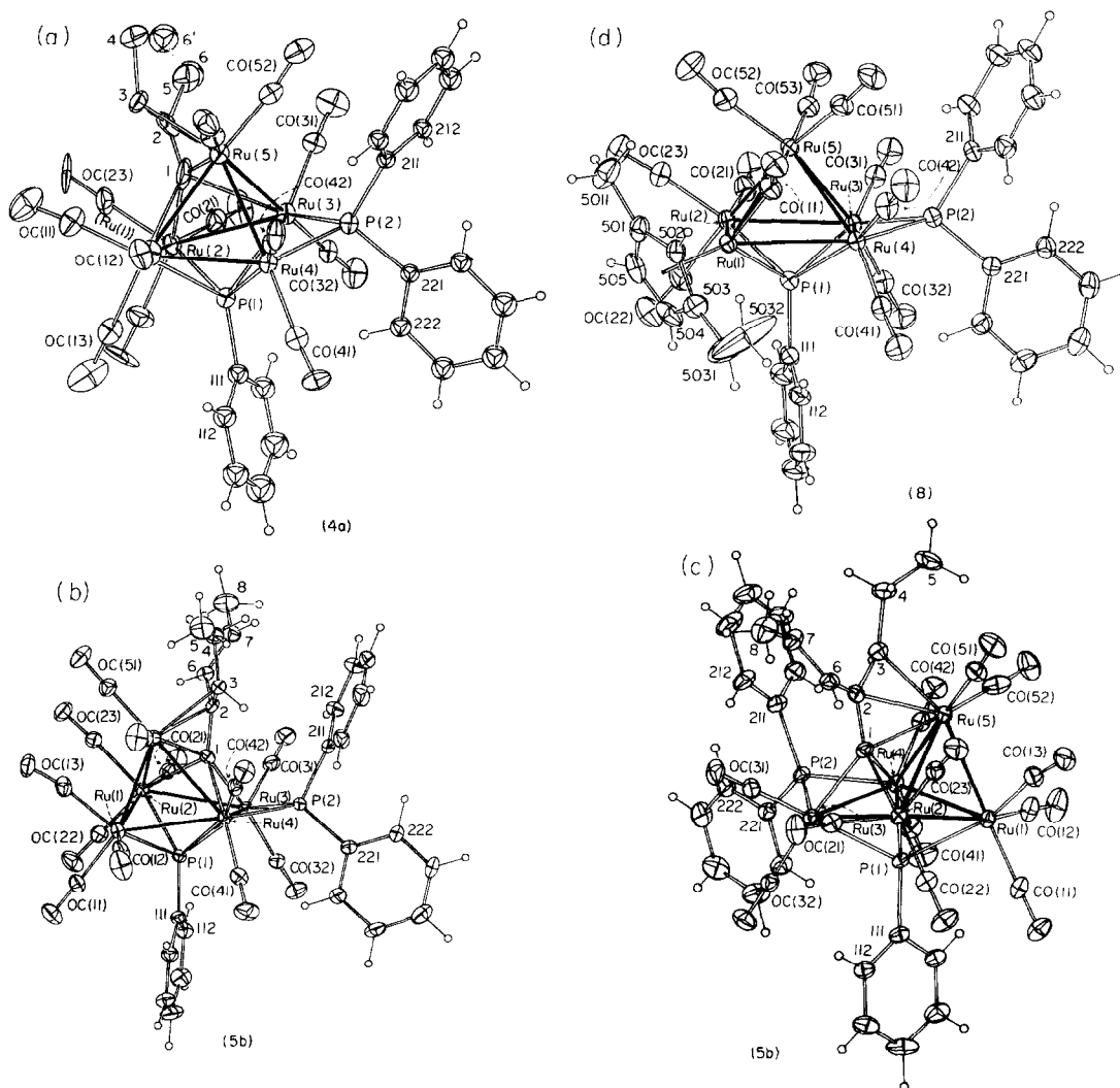
Fig. 1. (a) ORTEP diagram [23] of a molecule of \text{Ru}_5(\mu_4\text{-PPh})(\mu_4\text{-CC(CHCH}_2\text{)(CHMe)})(\mu\text{-PPh}_2)(\text{CO})_{12} ( 4a ), showing atom numbering scheme. Non-hydrogen atoms shown as 15% thermal ellipsoids; hydrogen atoms have arbitrary radii of 0.1 Å. (b) Plot of a molecule of \text{Ru}_5(\mu_4\text{-PPh})(\mu_4\text{-CC(CHCHMe)(CHEt)})(\mu\text{-PPh}_2)(\text{CO})_{12} ( 5b ), showing atom numbering scheme. (c) Alternative view of 5b showing the 'butterfly' configuration of the basal \text{Ru}_4 unit. (d) Plot of a molecule of \text{Ru}_5(\mu_4\text{-PPh})(\mu\text{-PPh}_2)(\mu\text{-CO})(\text{CO})_{10}(\eta^5\text{-C}_5\text{H}_3\text{Me-1-(CH=CH}_2\text{)-3}) ( 8 ), showing atom numbering scheme.
