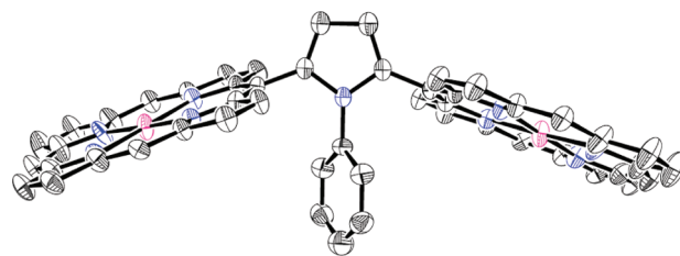
Figure 1. X-ray crystal structure of 2a . meso -Aryl groups and hydrogen atoms are omitted for clarity. The thermal ellipsoids were at 50% probability level.
