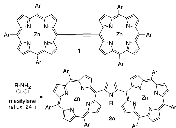
Scheme 1. Synthesis of 2a a
