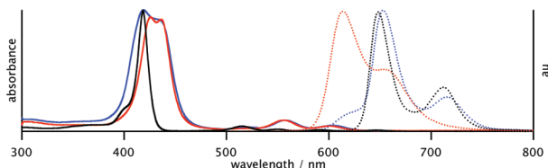
Figure 4. UV-vis absorption (left) and fluorescence (right) spectra in \text{CHCl}_3 (blue line = 4, red line = 2a, black line = TPP).
