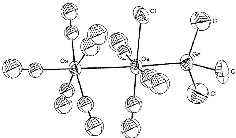
Fig. 1. Molecular structure of (\text{OC})_5\text{OsOs}(\text{CO})_3(\text{GeCl}_3)(\text{Cl}) .
