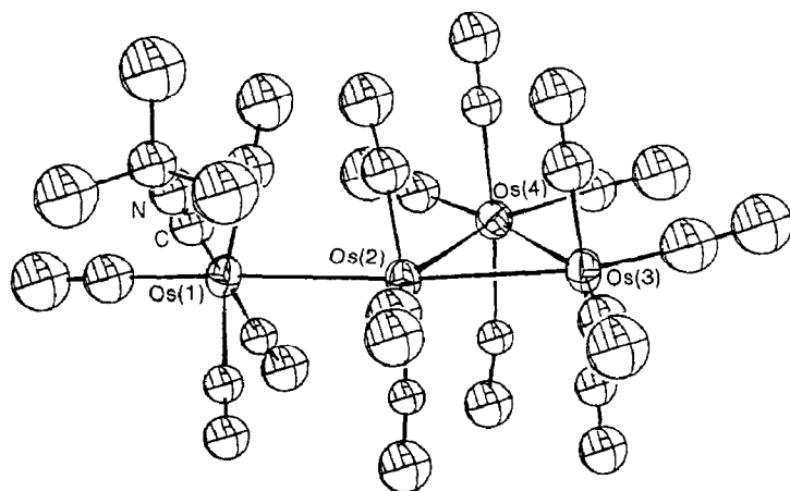
Fig. 11. Molecular structure of \text{Os}_4(\text{CO})_{15}(\text{CNBu}^t) ( 13 ).
