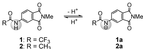
Scheme 1. Modification of Electronic Properties of 1 and 2
