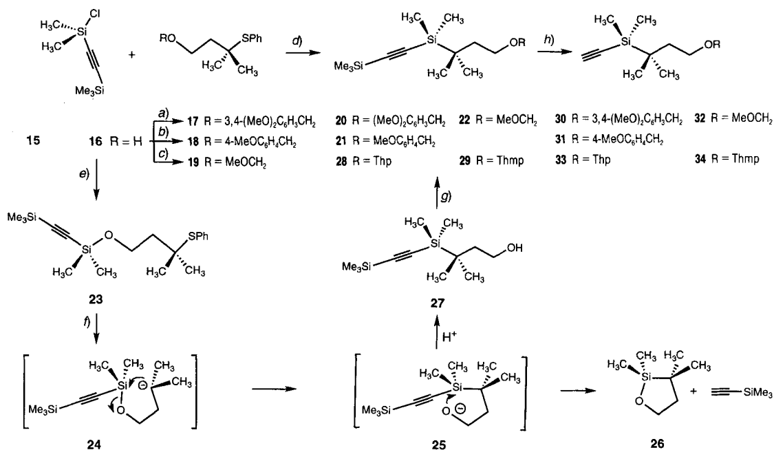
Scheme 3
