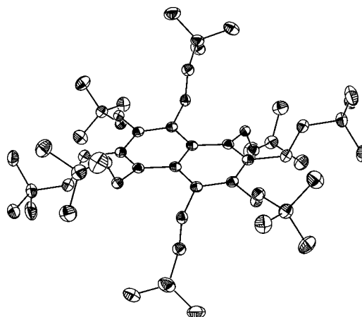
Figure 6. Structure of octakis-( tert -butylethenyl)naphthalene ( 27 ) in the crystal. [38]
