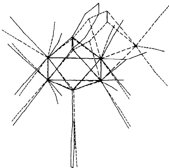
Fig. 5. Comparison of the non-hydrogen atom geometries of 2a and 3a, superimposed by least-squares fit of their \text{Ru}_4 units.
