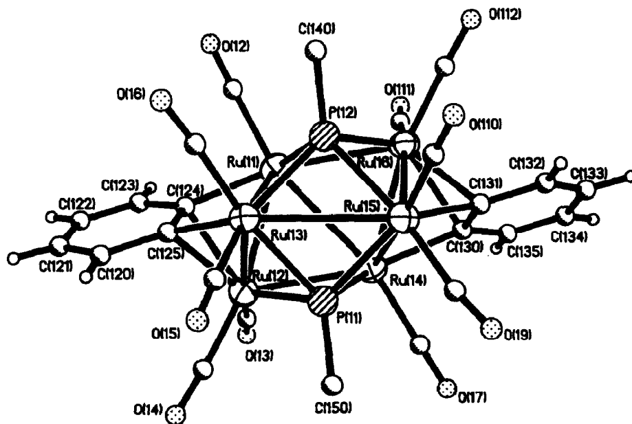
Fig. 4. Molecular structure of one of the two independent molecules of 11 , showing atom labelling scheme. Methyl group hydrogens have been omitted for clarity. Metal atoms are represented as ellipsoids enclosing 50% probability density, other atoms as spheres of arbitrary radii. Two carbonyl ligands, on Ru(11) and Ru(14), are obscured.
