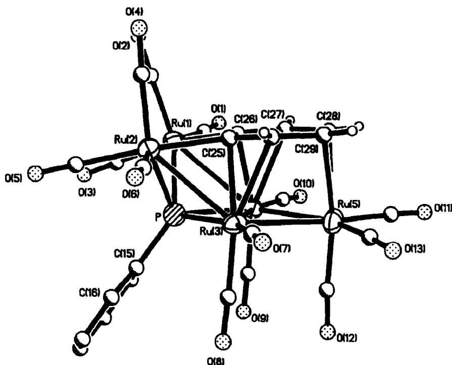
Fig. 3. Molecular structure of 3a , showing atom labelling scheme. Phenyl group hydrogens have been omitted for clarity. Metal atoms are represented as ellipsoids enclosing 50% probability density, other atoms as spheres of arbitrary radii. Ruthenium atom Ru(4) is partially obscured by Ru(3).
