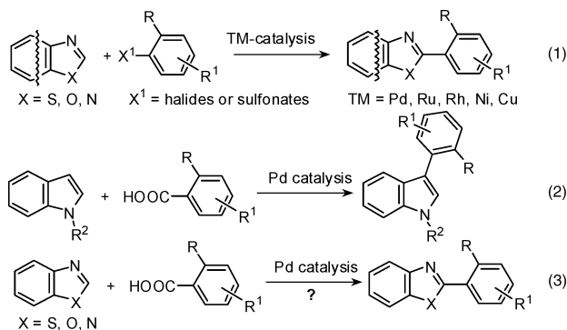
Scheme 1. Strategies for the Arylation of Heterocycles
