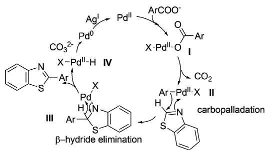
Scheme 2. Possible Mechanism for the Pd-Catalyzed Decarboxylative Arylation of Benzothiazole with Substituted Benzoic Acids
