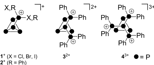
Chart 1. Cationic Phosphorus Cages
