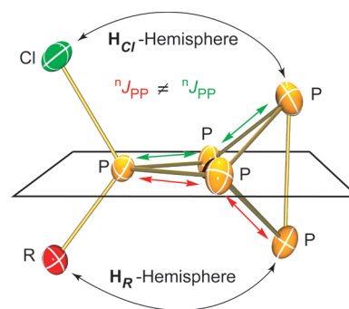
Figure 7. Definition of the \text{H}_{\text{Cl}} - and \text{H}_{\text{R}} -hemisphere in cages 21a–g ^{+} . The tetra-coordinate and bridging tricoordinate phosphorus atoms span a plane. The tricoordinate phosphorus atom above the plane lies within the \text{H}_{\text{Cl}} -hemisphere (marked by green dots, Figure 5), the phosphorus atom below in the \text{H}_{\text{R}} -hemisphere (marked by a yellow dots, Figure 5).
