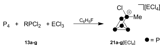
Scheme 3. Preparation of Compounds 21a-g [\text{ECl}_4] from \text{P}_4 , \text{RPCl}_2 , and \text{ECl}_3 in Fluorobenzene at RT ( \text{E} = \text{Al}, \text{Ga} )
