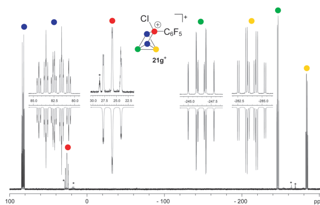
Figure 8. ^{31}\text{P}\{^1\text{H}\} NMR spectrum of cation 21g ^{+} ( \text{C}_6\text{D}_6 -capillary, \text{C}_6\text{H}_5\text{F} , 25 °C, 161.94 Hz). Signals assigned to unknown side-products are labeled with asterisks. Expansion (inset) show the experimental (up) and fitted 36 (down) spectra of cation 21g ^{+} .
