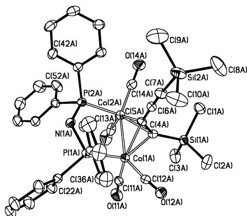
Fig. 2. ORTEP diagram of \text{Co}_2(\text{CO})_4(\text{dppa})_2(\mu\text{-}\eta^2\text{-Me}_3\text{SiC}_2\text{C}\equiv\text{CSiMe}_3) , 4 , (molecule 1) with 30% ellipsoids. H atoms have been removed for clarity.
