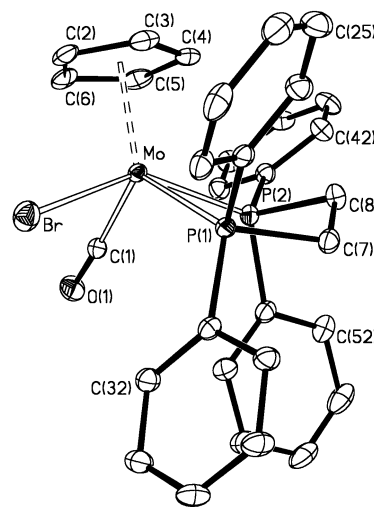
Fig. 1. ORTEP diagram of ( \eta^5\text{-C}_5\text{H}_5 )Mo(CO)(dppe)Br, 1a , with 30% ellipsoids. H atoms on the cyclopentadienyl and phenyl groups have been removed for clarity.
