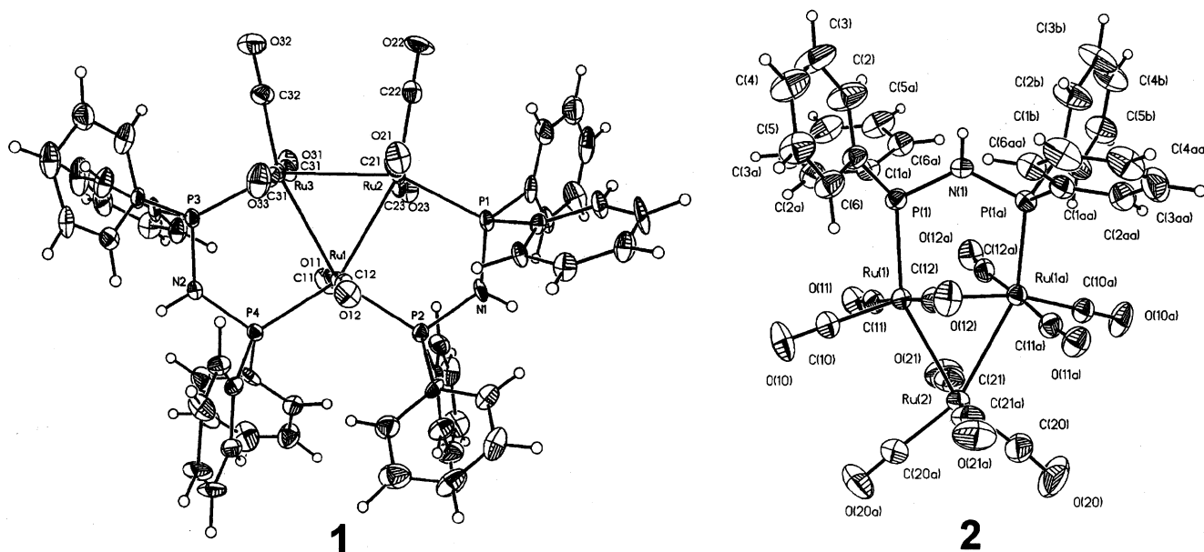
Fig. 1. Molecular structure of [\text{Ru}_3(\text{CO})_8(\text{dppa})_2] ( 1 ) and of [\text{Ru}_3(\text{CO})_{10}(\text{dppa})] ( 2 ).
