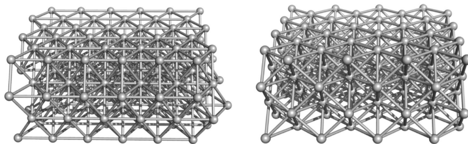
Figure 1. Pt(111) and Pt(100) supercells used for adsorption studies.
