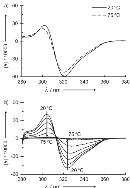
Figure 7. Temperature-dependent change of CD spectra of 8d in octane (a) and p -xylene (b) at 1.0 mM (0.01 cm width cell) at 20, 30, 40, 50, 60, 70, and 75 °C.
