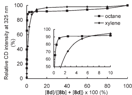
Figure 12. Plots of relative CD intensity at 325 nm ( CD_{obs}/CD_{100\text{ mol \% of } \mathbf{3d}} \times 100 ) vs mole percentage of 8b ( [\mathbf{8d}]/([\mathbf{8b}] + [\mathbf{8d}]) \times 100 ) for the mixture of 8b and 8d in octane and p -xylene. The total concentration of 8b and 8d was kept at 1.0 mm.
