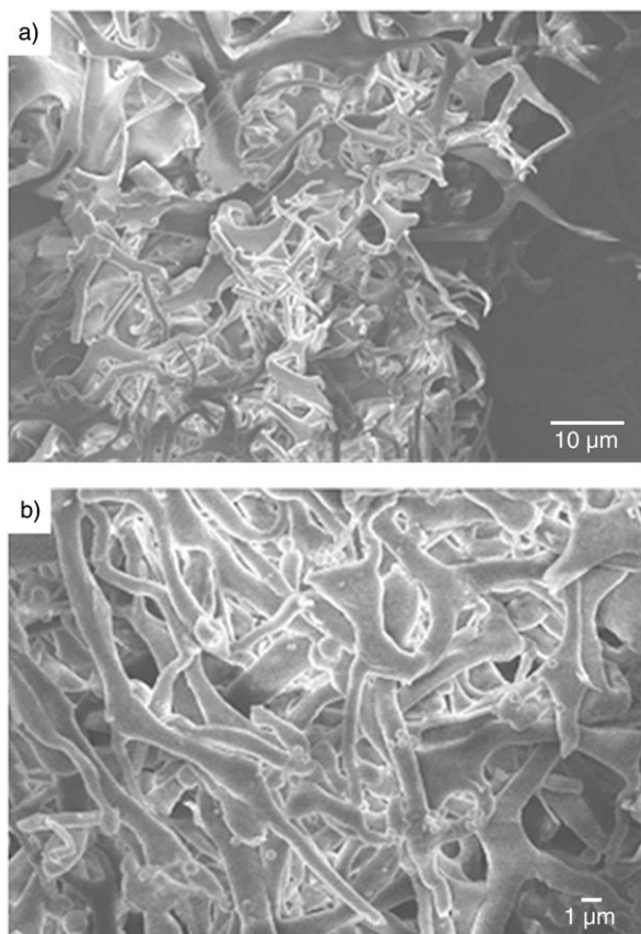
Figure 1. SEM images of cyclohexane xerogels of 8b (a) and 8d (b), prepared at -15^{\circ}\text{C}/0.1 Torr.
