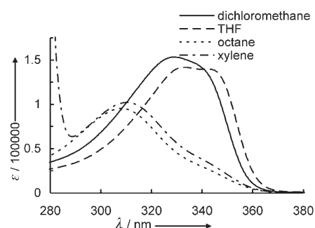
Figure 2. UV/Vis spectra of 8b in octane, p -xylene, dichloromethane, and THF at 1.0 mm (0.01 cm width cell) at 20^{\circ}\text{C} .
