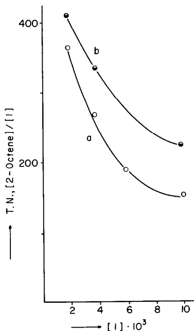
Fig. 6. Plots of TN versus cluster 1 concentration for the 1-octene isomerization reaction at 70°C using dioxane (0.8 ml)/benzene (5 ml), 1-octene (2.35 ml, 1.50 M) and (\text{EtO})_3\text{SiH} (1.85 ml, 1.00 M). Measurements taken after 11 min (a) and 90 min (b).
