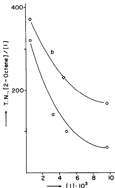
Fig. 5. Plots of TN values versus cluster 1 concentration for the 1-octene isomerization reaction at 60^\circ\text{C} using dioxane (0.8 ml)/benzene (5 ml), 1-octene (2.35 ml, 1.50 M) and (\text{EtO})_3\text{SiH} (1.85 ml, 1.00 M). Measurements taken after 11 min (a), and 60 min (b).
