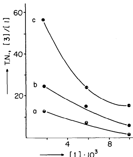
Fig. 8. Plots of TN versus cluster 1 concentration for the by-product 3 production at 70°C using dioxane (0.8 ml)/benzene (5 ml), 1-octene (2.35 ml, 1.50 M) and (\text{EtO})_3\text{SiH} (1.85 ml, 1.00 M). Measurements taken after 5 min (a), 11 min (b) and 60 min (c).
