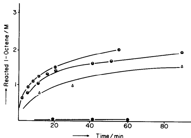
Fig. 3. Reaction profiles showing the effect of initial (\text{EtO})_3\text{SiH} concentration on the rate of 1-octene isomerization reaction. Conditions: in dioxane (variable to make total volume 10 ml)/benzene (5 ml) using 1 (0.0160 g, 2.50 \times 10^{-5} mol) and 1-octene (2.35 ml, 1.50 M) at 60^\circ\text{C} . (\text{EtO})_3\text{SiH} concentrations: \bullet , 0.00 M; \triangle , 0.34 M; \bullet , 0.50 M; \odot , 1.00 M.
