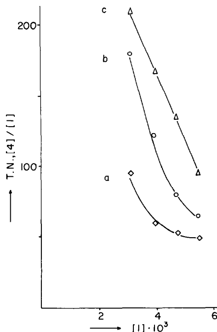
Fig. 9. Plots of TN versus cluster 1 concentration for the acetophenone hydrosilylation. Dioxane (0.8 ml)/benzene (5 ml), 1-octene (2.35 ml, 1.50 M) and (\text{EtO})_3\text{SiH} (1.85 ml, 1.00 M). Measurements taken after 30 min (a), 90 min (b) and 140 min (c). T = 70^\circ\text{C} .
