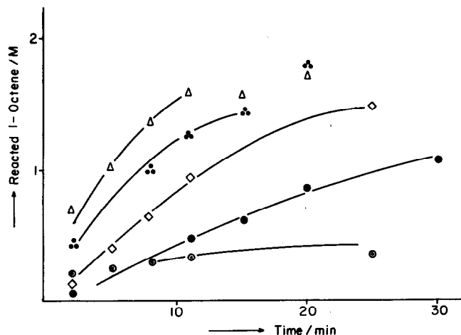
Fig. 4. Reaction profiles showing the effect of initial (\text{EtO})_3\text{SiH} concentration on rate of 1-octene isomerization reaction. Conditions: in dioxane (variable to make total volume 10 ml)/benzene (5 ml) using 1 (0.0630 g, 9.85 \times 10^{-5} mol) and 1-octene (2.35 ml, 1.50 M) at 70^\circ\text{C} . (\text{EtO})_3\text{SiH} concentrations: \circ , 0.00 M; \bullet , 0.33 M; \bullet , 0.50 M; \triangle , 1.00 M.
