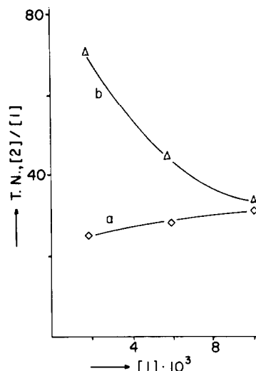
Fig. 7. Plots of TN versus cluster 1 concentration for the olefin hydrosilylation reaction at 70°C using dioxane (0.8 ml)/benzene (5 ml), 1-octene (2.35 ml, 1.50 M) and (\text{EtO})_3\text{SiH} (1.85 ml, 1.00 M). Measurements taken after 11 min (a) and 30 min (b).
