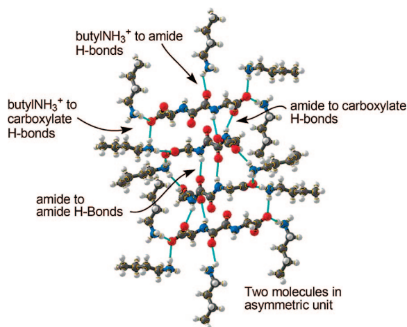
Figure 7. Crystal structure of (butylNH 3 ) 2 og.
