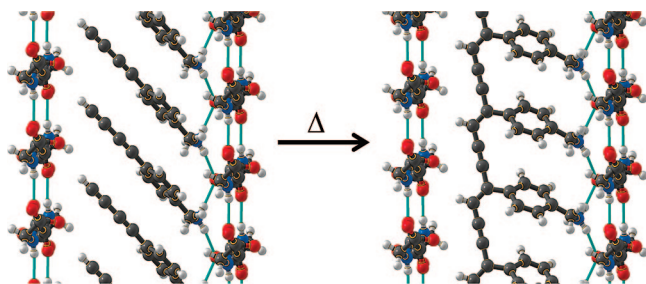
Figure 14. On the left is a view of the crystal structure of the (\text{DABzNH}_3)_2\text{og} salt. The right-hand side shows a similar view of the polymerized structure. The same crystal was used for both experiments.
