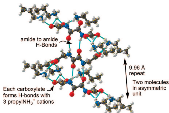
Figure 6. Crystal structure of (propylNH 3 ) 2 og.
