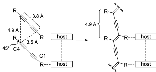
Figure 1. Topochemical requirements for diacetylene polymerization and the host-guest strategy of aligning diacetylenes for such requirements.
