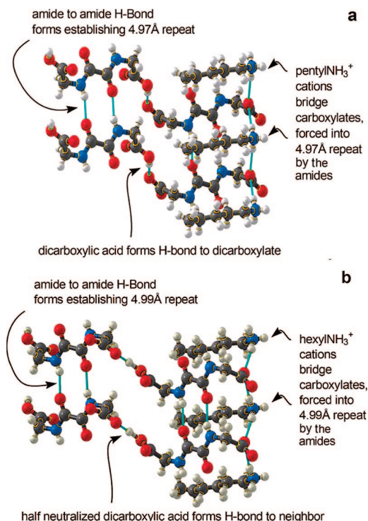
Figure 8. Crystal structures of (a) (pentylNH 3 ) 2 og·H 2 og and (b) (hexylNH 3 ) 2 Hog.
