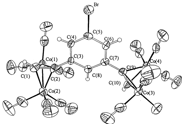
Fig. 3. ORTEX drawing of the molecular structure of 16 (thermal ellipsoids have been drawn at 40% probability level, hydrogen atoms have been omitted for clarity).
