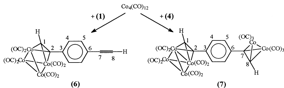
Scheme 2. Schematic representation of the complexes containing {Co 4 (CO) 8 ( \mu -CO) 2 } units. The bridging carbonyl ligands have been removed for clarity. The atom labels are consistent with the NMR assignments.
