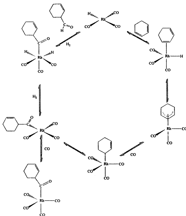
Fig. 7. Proposed unicyclic homogeneous rhodium catalytic cycle for the hydroformylation of conjugated dienes under low conversion, with presence of \eta^3 allyl rhodium tricarbonyl species, \sigma allyl rhodium tetracarbonyl species and acyl rhodium tetracarbonyl species (R = alkenyl).
